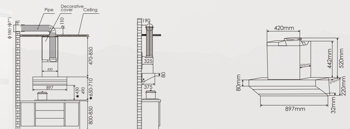
Installation Diagram
