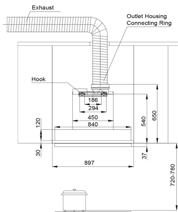
Installation diagram (★ is the distance from the wall)
